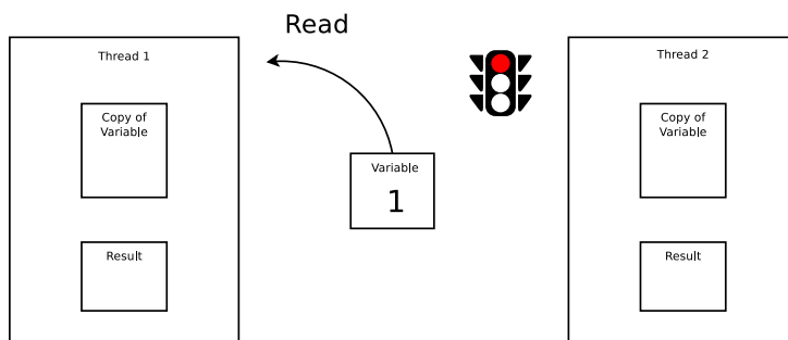
Figure 121: How mutex works (2/8)
